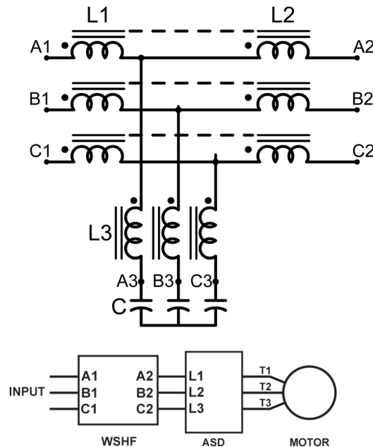
Fig. 1: Lineator AUHF schematic and connection diagram
